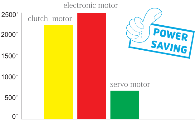
2 71% power saving 750W servo motor, with stronger penetration, high efficiency and energy saving
